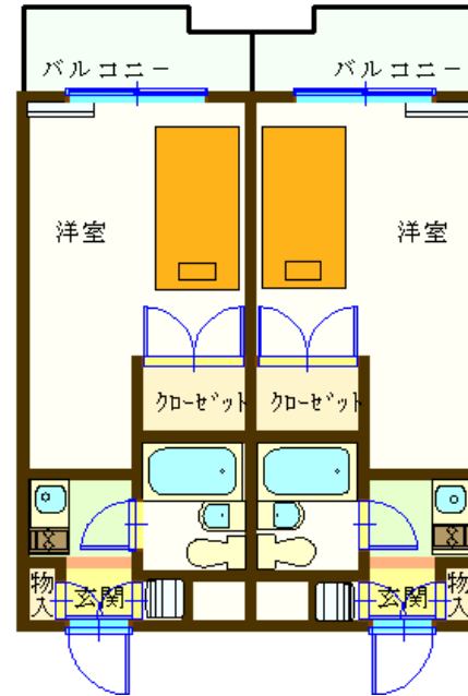
Floor plans
